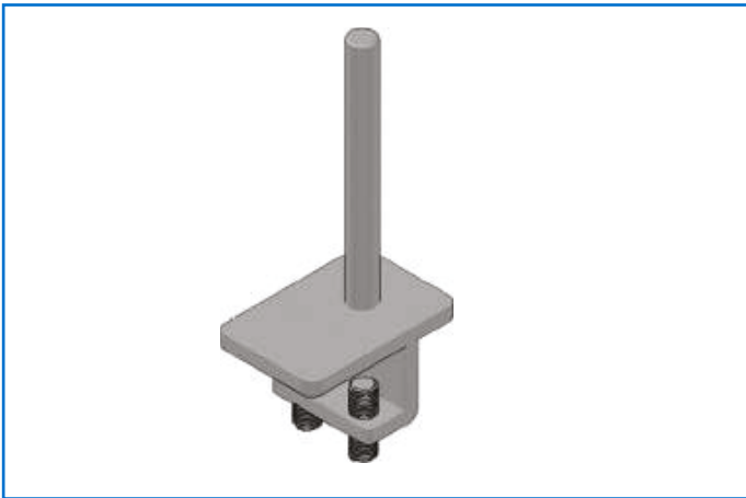
DTB2 25mm Clamp bracket with 20mm underhang Supplied with 2 x 7mm grub screws
