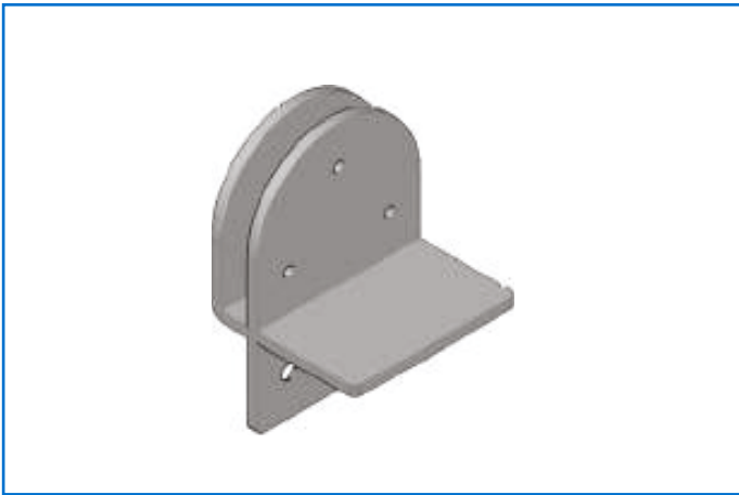
DTBP/S 30mm Perspex screw bracket Supplied with 3 x 3mm grub screws
